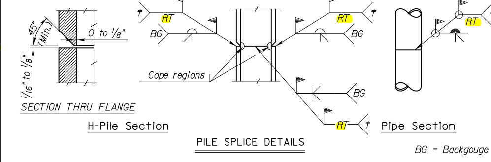
SECTION THRU FLANGE H-Pile Section PIPE SPLICE DETAILS Pipe Section BG = Backgouge
