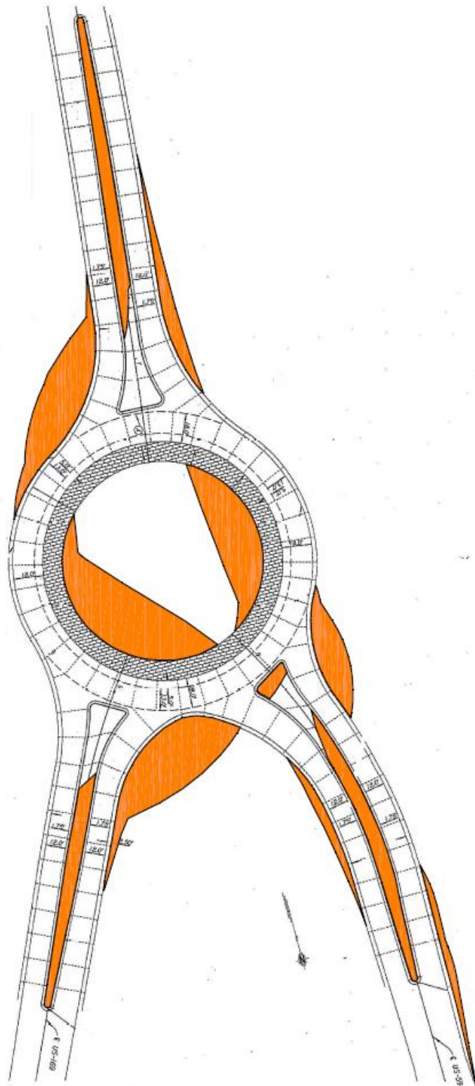
FIGURE 6.27 Extra Traversable Area/Truck Apron Required for Garnett Roundabout Based on Vehicle Simulations in Figure 6.26
