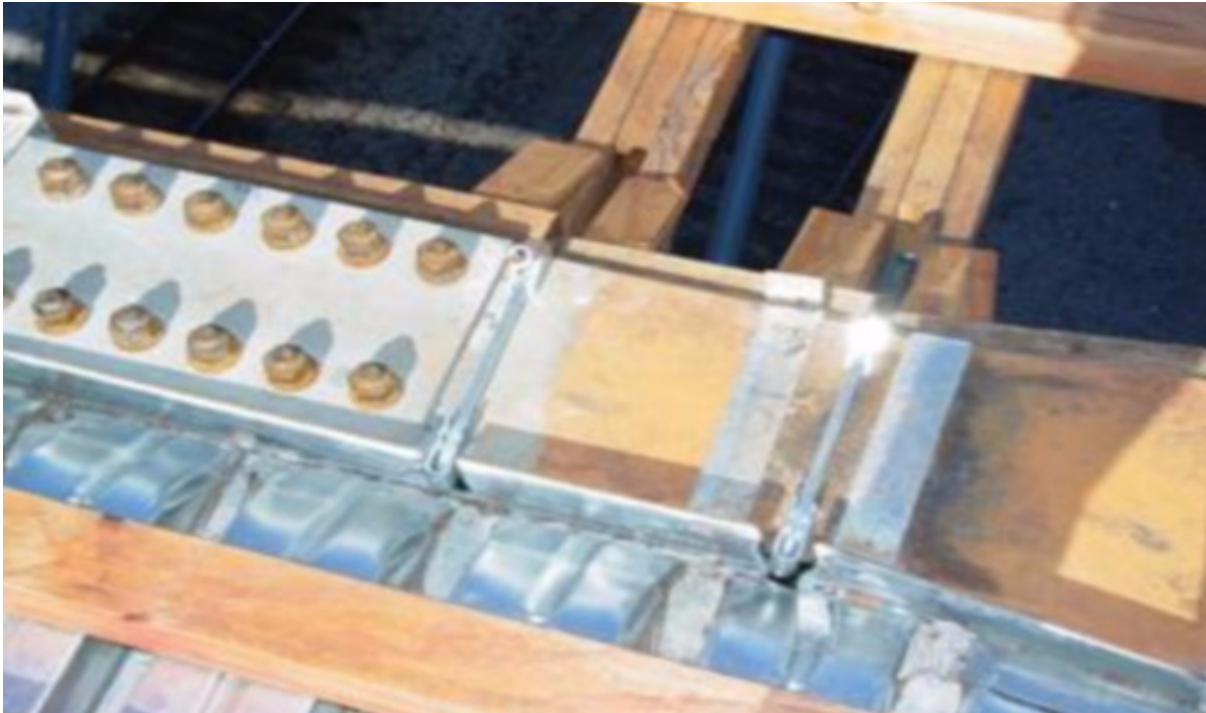
Figure 13: Steel SIP Forms and Welded Support Hangers
