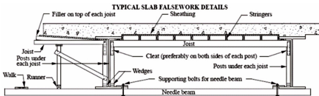
Figure 7: Needle Beam System Components
