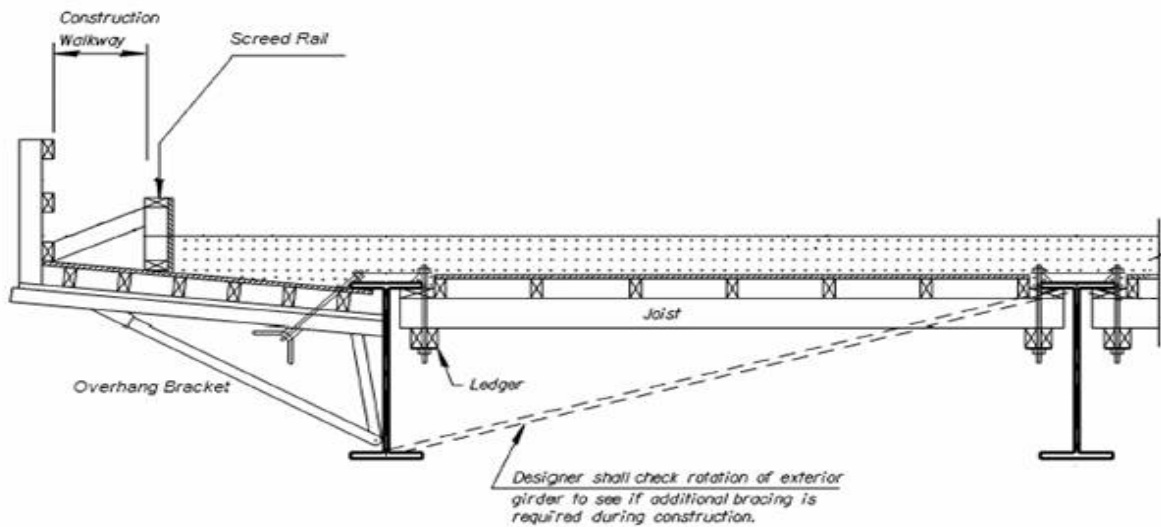
Typical Falsework for Girder Bridges
