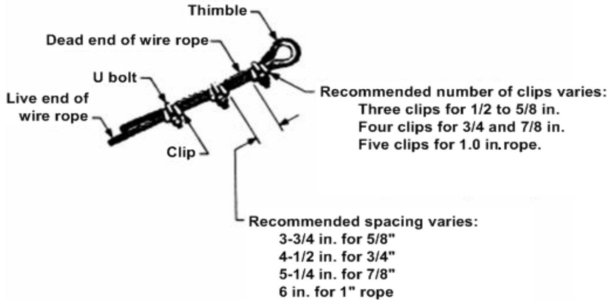
Figure 5: Cable Bracing Detail
