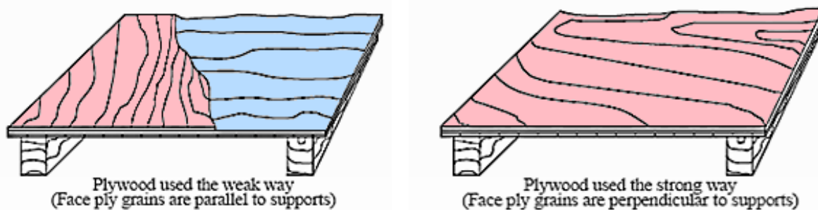
Figure 3: Plywood Grain Orientation
