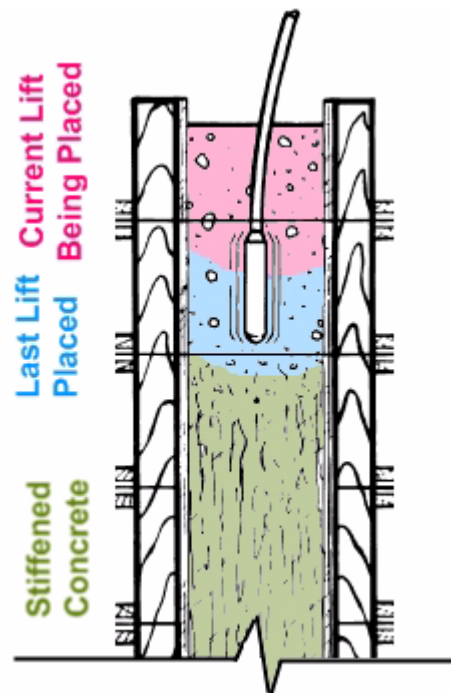
Figure 21: Placement and Initial Set of Concrete
