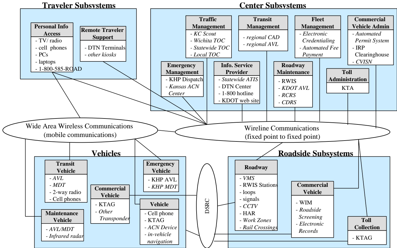
Figure 3: Kansas Statewide ITS Architecture
